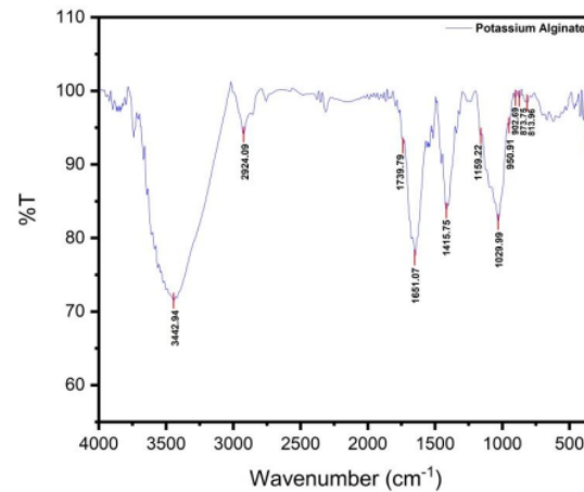
Figure 1. Infrared spectrum of potassium alginate extracted from Sargassum polycystum .
